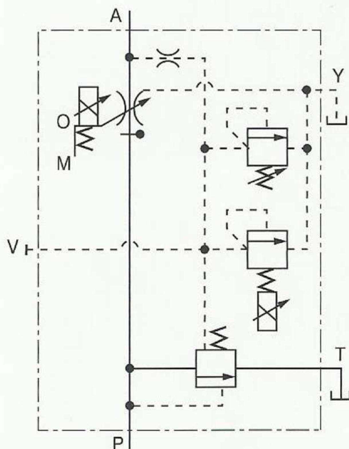
WITH PROPORTIONAL PILOT RELIEF VALVE
