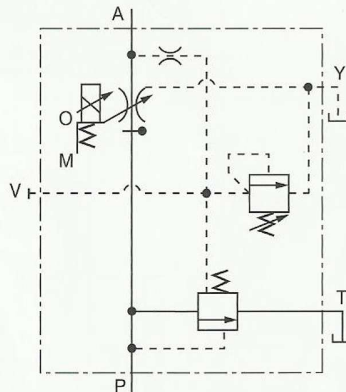
WITHOUT PROPORTIONAL PILOT RELIEF VALVE
